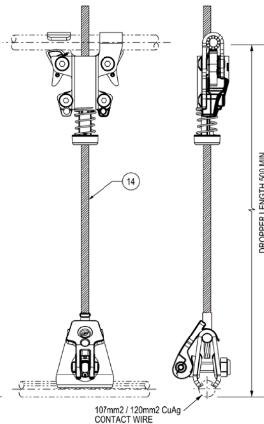
REF NO. C99/F01/006 GRIPPLE DROPPER
