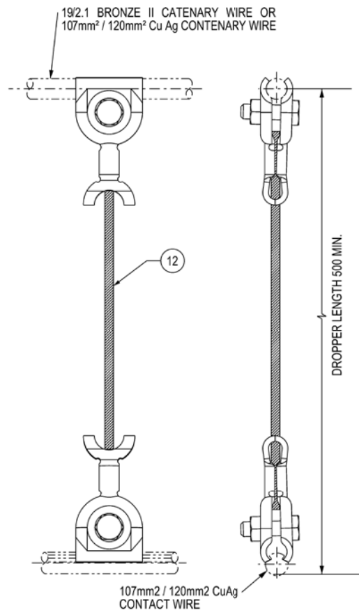
REF NO. C99/F01/004 KRUCH DROPPER
