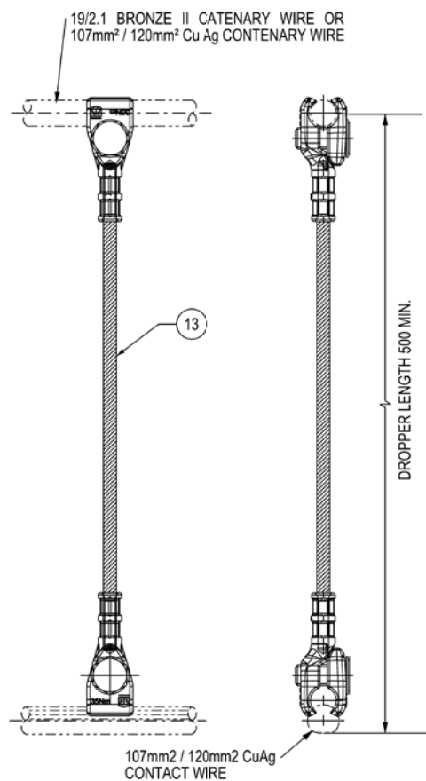
REF NO. C99/F01/005 BONOMI BE1307 DROPPER
