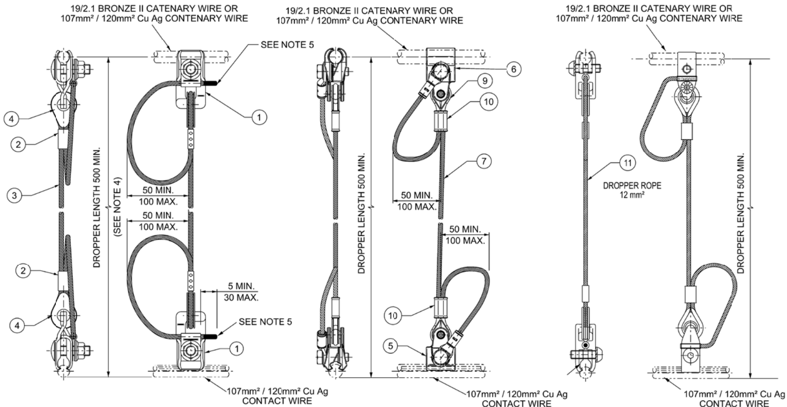
REF NO. C99/F01/001 ARTHUR FLURY DROPPER
